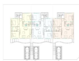
PENTHOUSE - PLANTA ALZA
